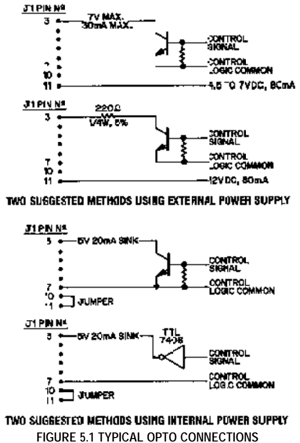
FIGURE 5.1 TYPICAL OPTO CONNECTIONS
