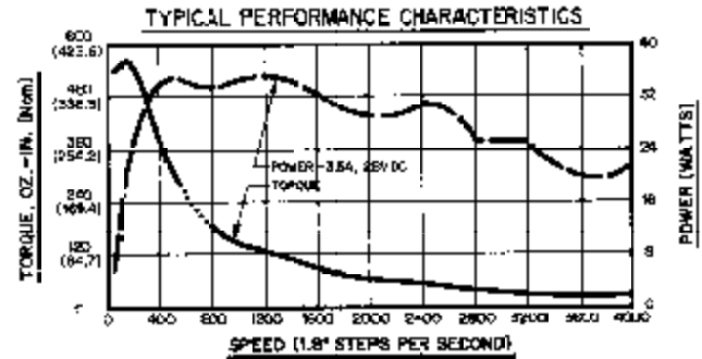
SERIES CONNECTION MO93-FD0011 MOTOR
