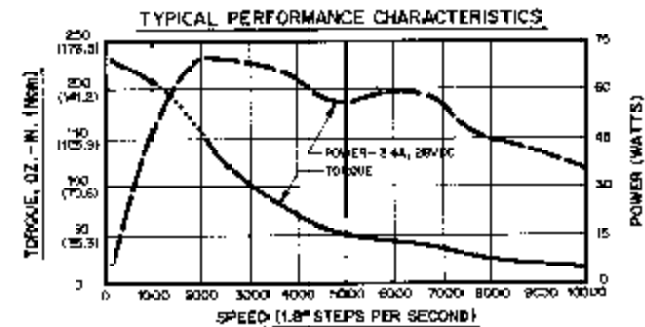
PARALLEL CONNECTION MO93-FD0014 MOTOR
