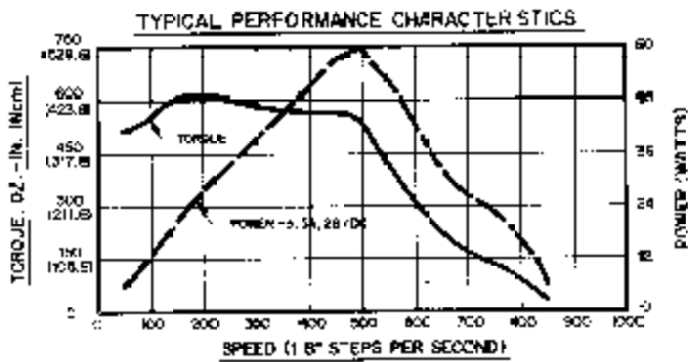
SERIES CONNECTION M112-FJ8030 MOTOR
